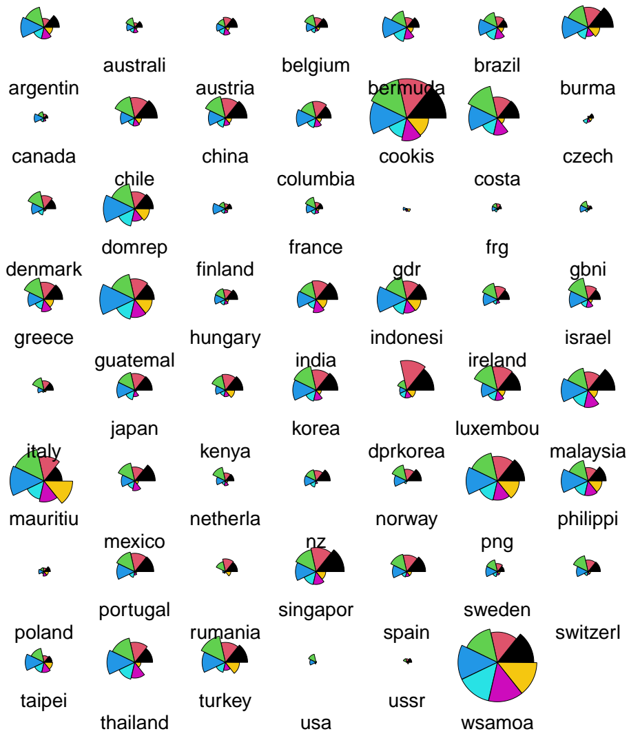
Radar plot.
