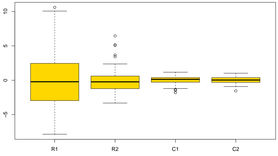
Box plot.
