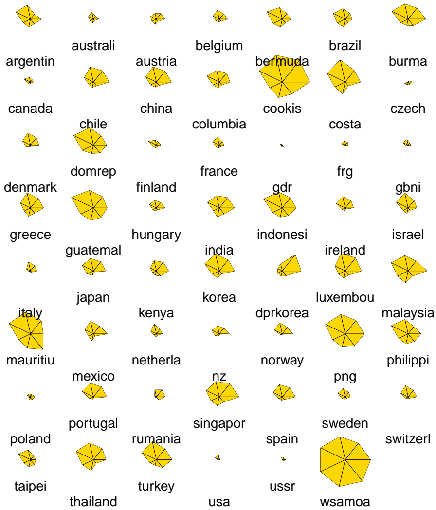
Star plot.
